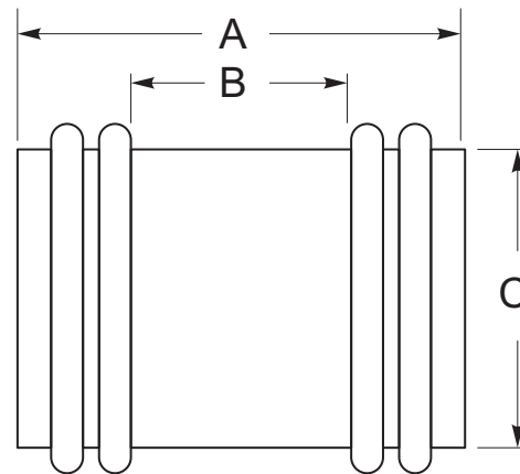
3 1/2" to 6 I.P.S. 4" to 6 N.C.T.
